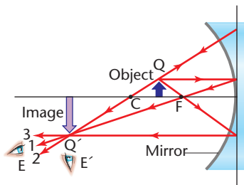
FIGURE 18–7 To the eye at E, it appears that there is an object at Q' blocking the view of the mirror. However, if the eye moves to E' and looks toward Q', the object disappears because there is no light reflected from Q' to E'.
